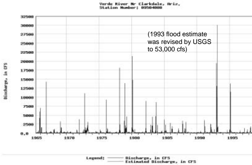
Figure 15. Daily mean streamflow at the Verde River near Clarkdale, 1965-1999 (USGS 1999).
